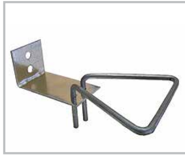
P-312 / P-316 ANCRAGE AJUSTABLE DOUBLE (2)
